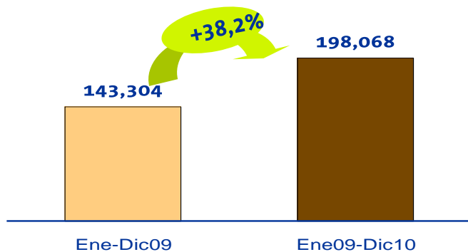
CAPEX (Mills$)
